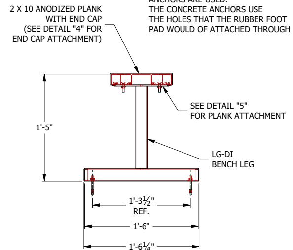
CONCRETE ANCHOR OPTION SEE DETAIL "3"
